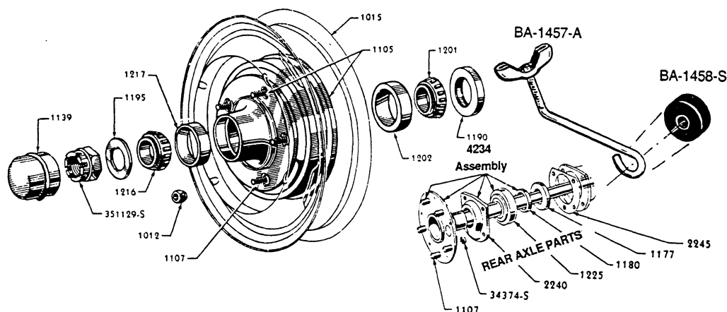
HUB CAP B7A-1130-B
